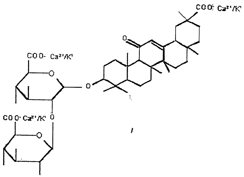
Glycyrrhizin = Ca 2+ & K + salts of Glycyrrhizinic acid
